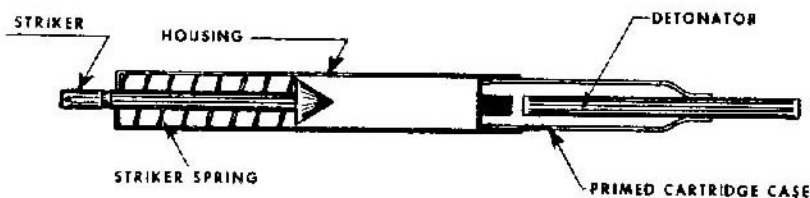
Figure 26 (UNCLASSIFIED). FLN improvised fuze (U).
